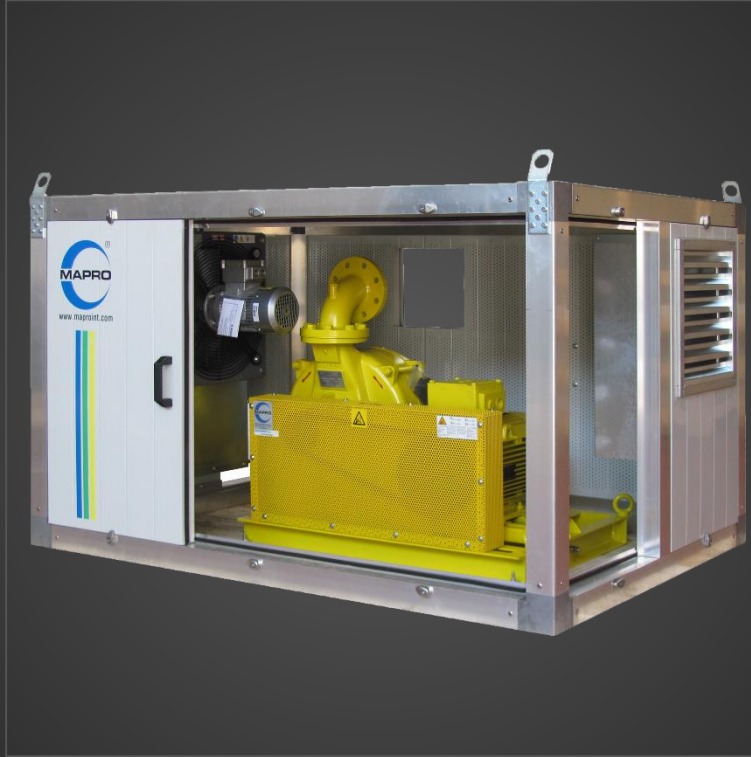
BELT-DRIVE VERSION WITH HORIZONTAL OUTLET AND ACOUSTIC ENCLOSURE
